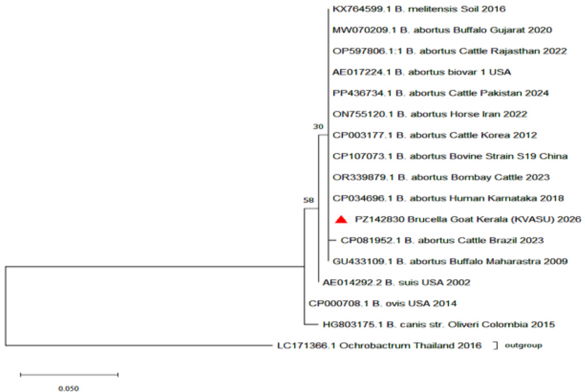
Fig. 2. Maximum-Likelihood phylogenetic tree of Brucella isolates based on IS711 sequences. The tree was constructed using the Tamura 3-parameter model with Ochrobactrum (LC171366.1) as the outgroup. Bootstrap values are shown at the nodes. The scale bar represents 0.050 substitutions per site. The red triangle indicates the Brucella isolate (PZ142830) identified in the present study.
