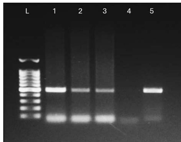
Fig. 1: Representative agarose gel electrophoresis of PCR amplification of IS711 region of Brucella abortus (498 bp). Lane L: 100 bp DNA ladder; lanes 1-3: positive samples; lane 4: negative control; lane 5: positive control.
