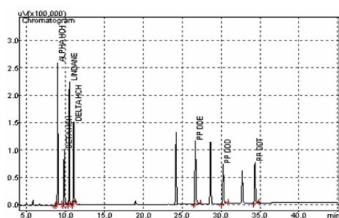
Fig.2. Chromatogram of Blood sample
